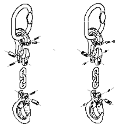
DISMOUNTABLE CONNECTIONS
